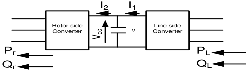
Figure 3: Power flow through dc-link element
