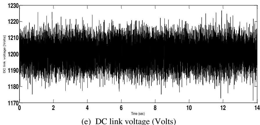
Figure 7: Performance of the proposed DFIG driven by a wind turbine system with linear bi-directional variation of wind speed
