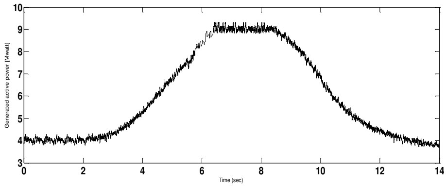
(c) Generated active power (Mwatt)
