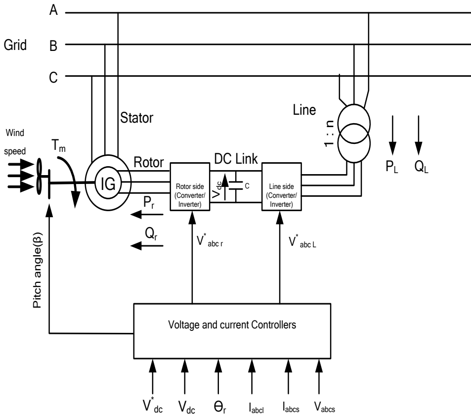
Figure 1: Doubly-fed induction Generator driven by a wind turbine System
