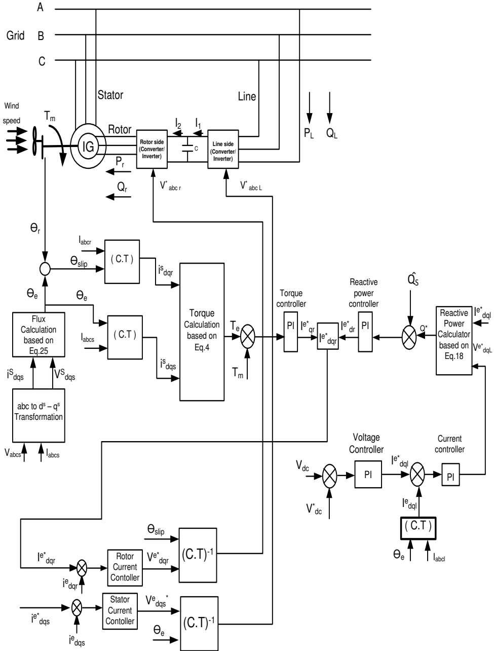
Figure 4: Proposed control scheme of the DFIG driven by a wind turbine based on field orientation
