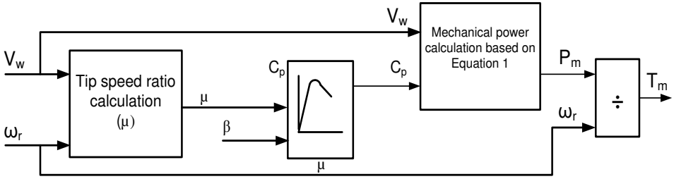
Figure 2: Wind turbine control system
