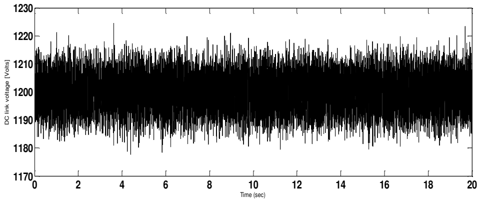
(e) DC link voltage (Volts)
