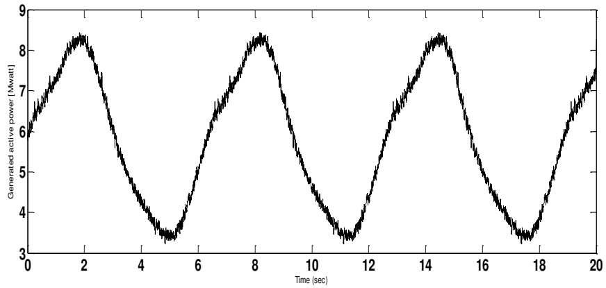
(c) Generated active power (Mwatt)
