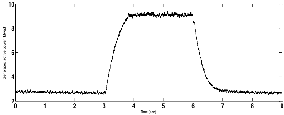
(c) Generated active power (Mwatt)
