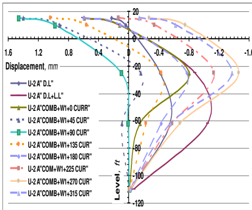
(c) U 2 for Leg A
