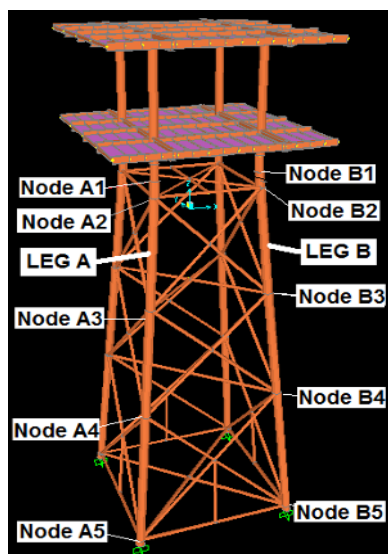
Fig. 4 Finite element model
