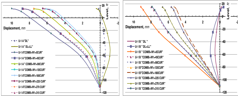
(a) U 1 for Leg A
