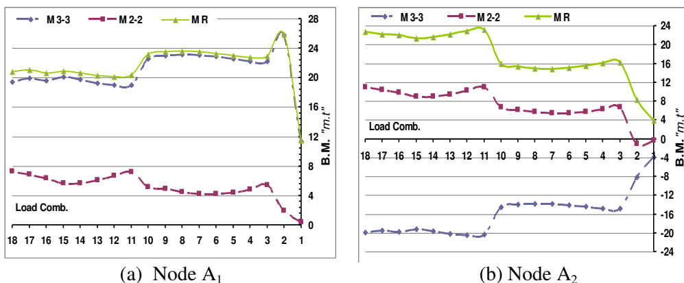
(a) Node A 1 (b) Node A 2 Fig. 11 the variation of the bending moment response with the variation of loadings
