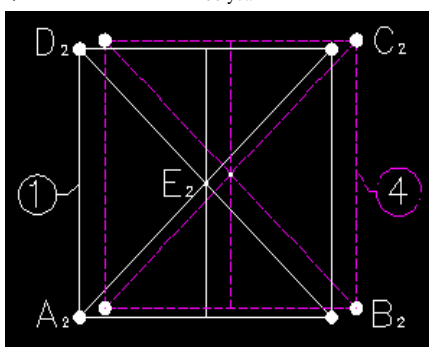
(c) DL + LL + W_{100\text{ year}} + 90^\circ current
