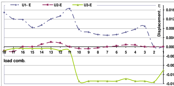
Fig. 9 The variation of Displacements of jacket center node E 2 at level (+10 ft) for different Load Combinations
