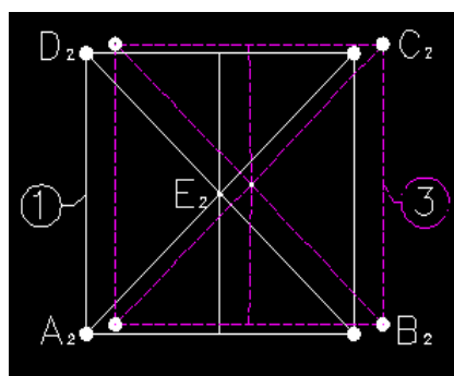
(b) DL + LL + W_{100\text{ year}} + 45^\circ current
