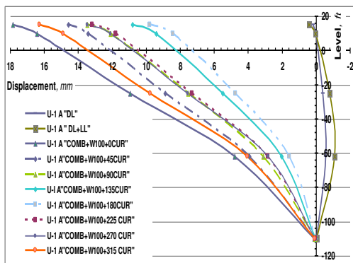
(a) U 1 for Leg A
