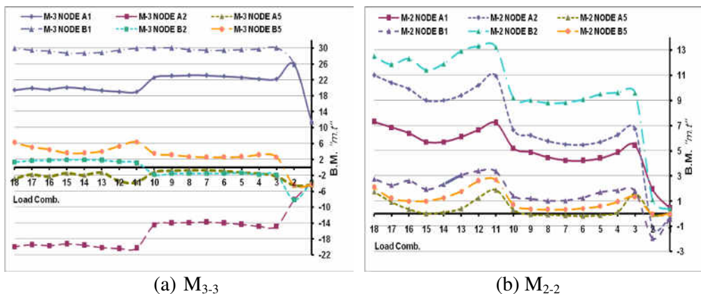
(a) M 3-3 (b) M 2-2 Fig. 12 Bending moment response with load combinations for different nodes
