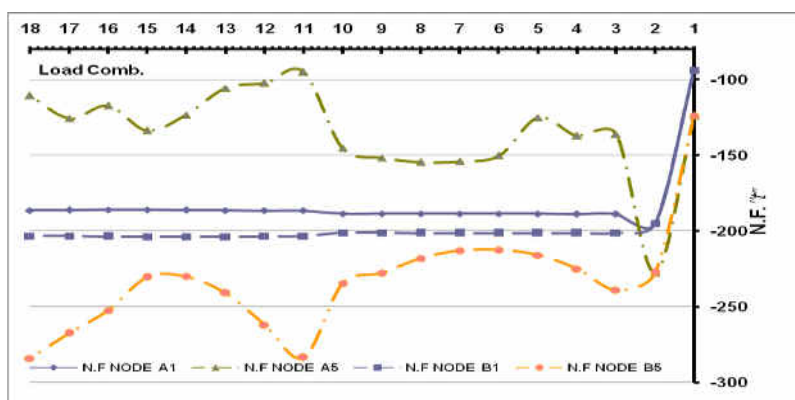
Fig. 13 Normal Force response "N.F." with load combinations for different nodes
