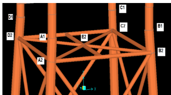
Fig. 5 Jacket - deck connection nodes at level (+10 ft)
